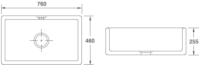
W:760 x D:460 x H:255mm
