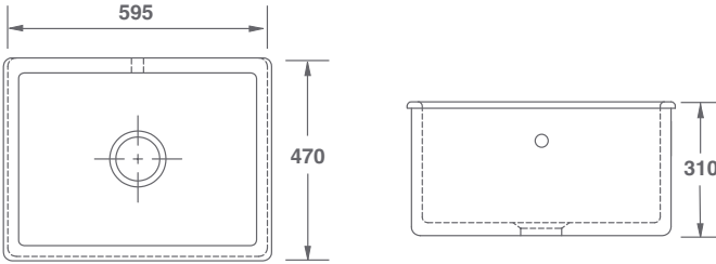
W:595 x D:470 x H:310mm
