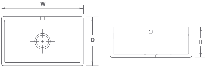
600 – W:595 x D:460 x H:255mm 800 – W:762 x D:457 x H:284mm
